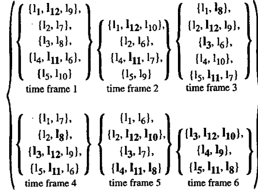
Fig. 7. A liquid schedule for the collective traffic shown in Fig. 1. Bold links in a time frame indicate bottlenecks in the reduced traffic.
