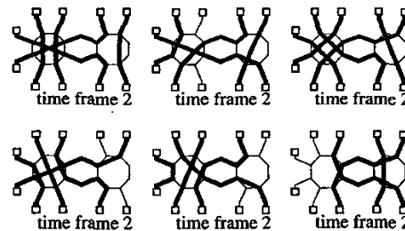
Fig. 3. An optimal schedule (6 time frames).
