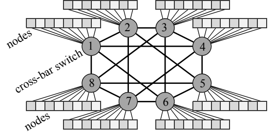
Fig. 8. Architecture of the T1 cluster computer interconnected by a high performance wormhole switch fabric.
