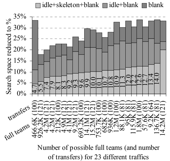
Fig. 5. Search space reduction obtained by idle+skeleton+blank optimization steps.
