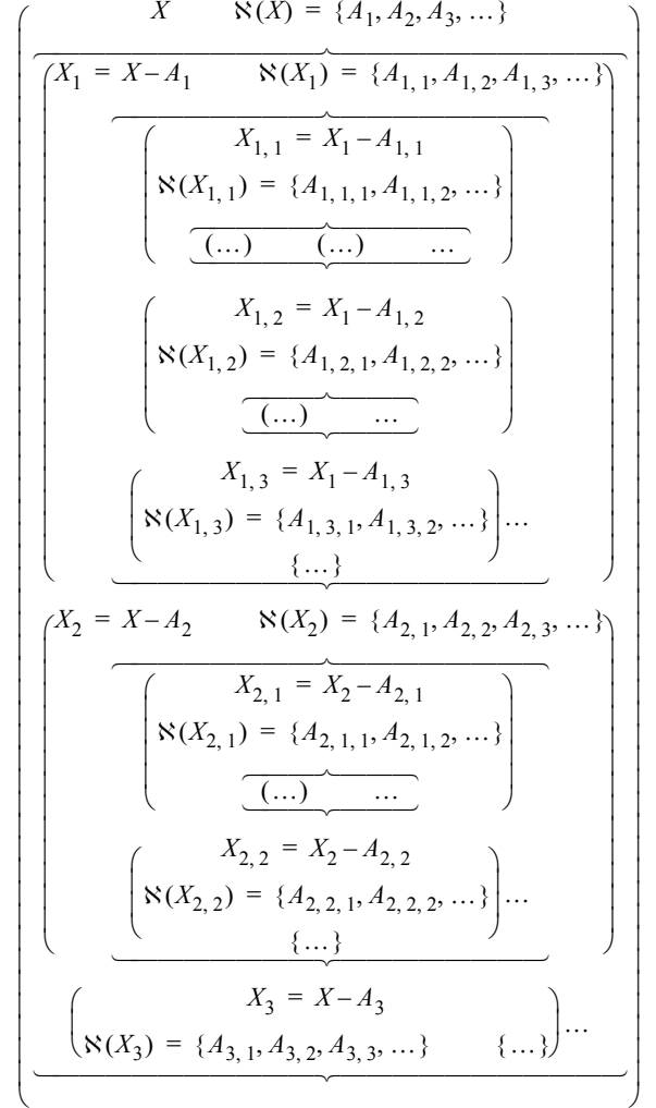
Fig. 7. Liquid schedule search tree. X_{i_1 i_2 \dots i_n} denotes a reduced subtraffic at the layer n + 1 of the tree and A_{i_1 i_2 \dots i_n i_{n+1}} denotes a candidate for the time frame n + 1 . The operator \aleph applied to a subtraffic X_{sub} represents the set of all possible candidates for a time frame at the present stage.
