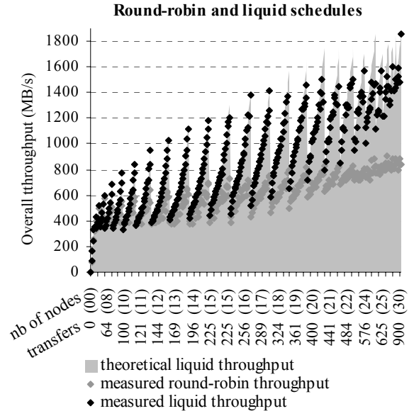
Fig. 9. Theoretical liquid throughputs and measured throughputs for traffics scheduled according to round-robin and liquid schedules.
