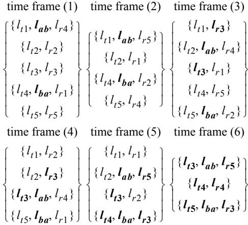
Fig. 6. The time frames of a liquid schedule of the collective traffic shown in Fig. 1.
